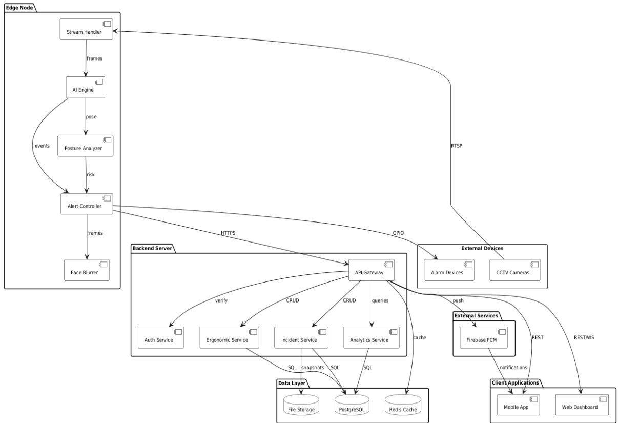
Figure [14] – Component Diagram
